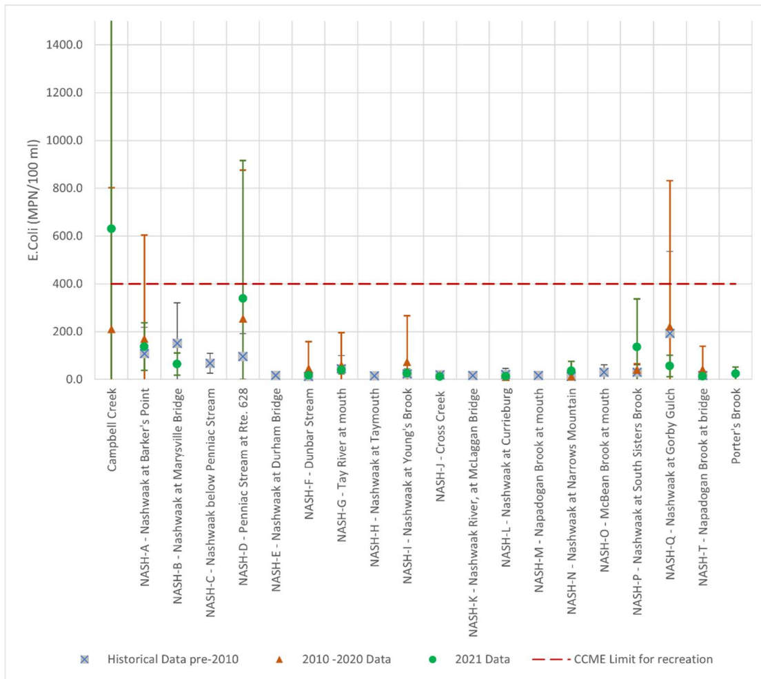
Figure 11 Mean E. coli contents (MPN/100 mL) per site in the watershed. Error bars represent standard deviation. The CCME limit is 400 MPN/ 100 mL for a single grab sample.
