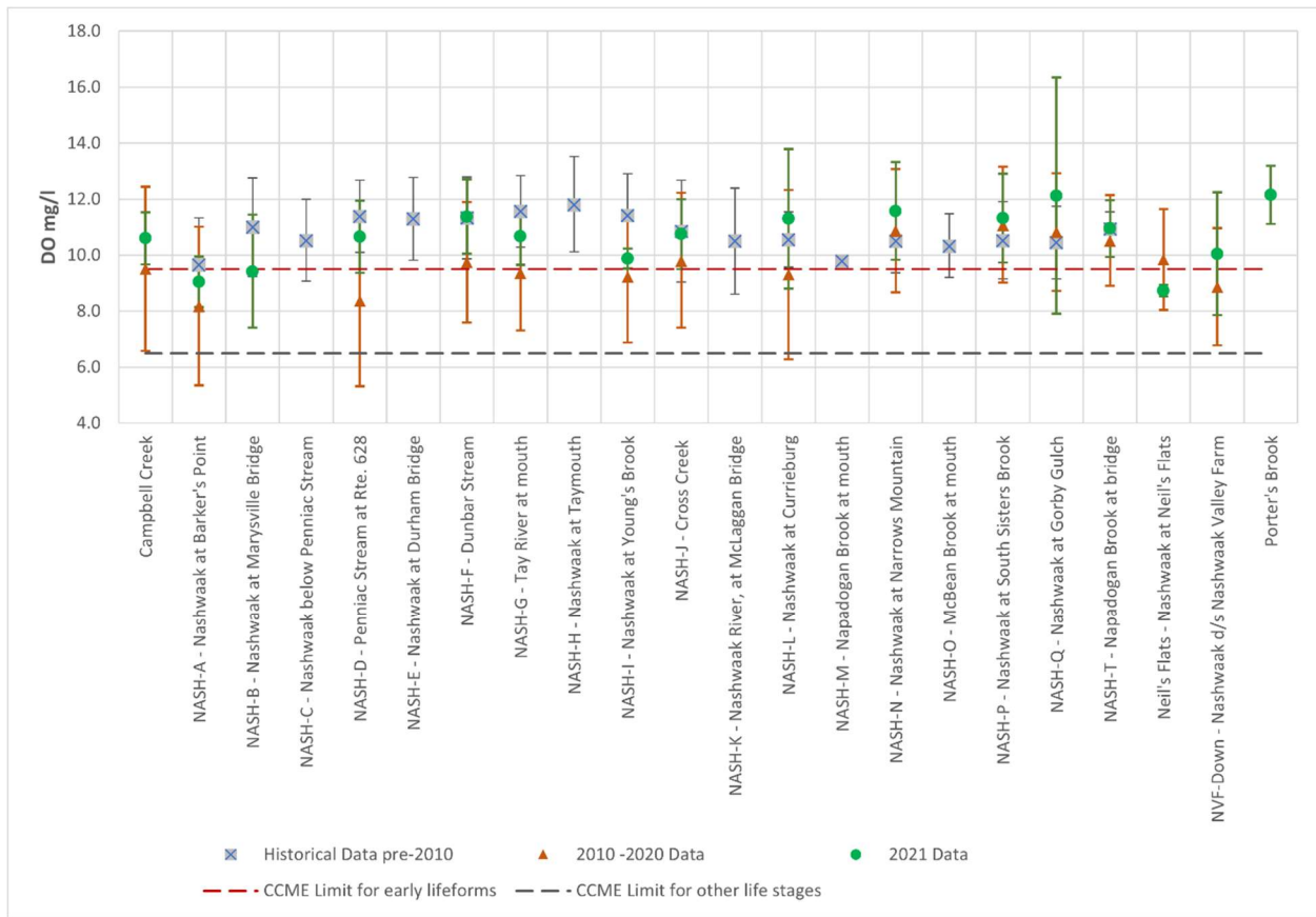
Figure 8 Mean dissolved oxygen content (mg/L) per site. Error bars represent standard deviation. Dashed lines indicate CCME limits for early life forms (9.5 mg/L) and all other life stages (6.5 mg/L).
