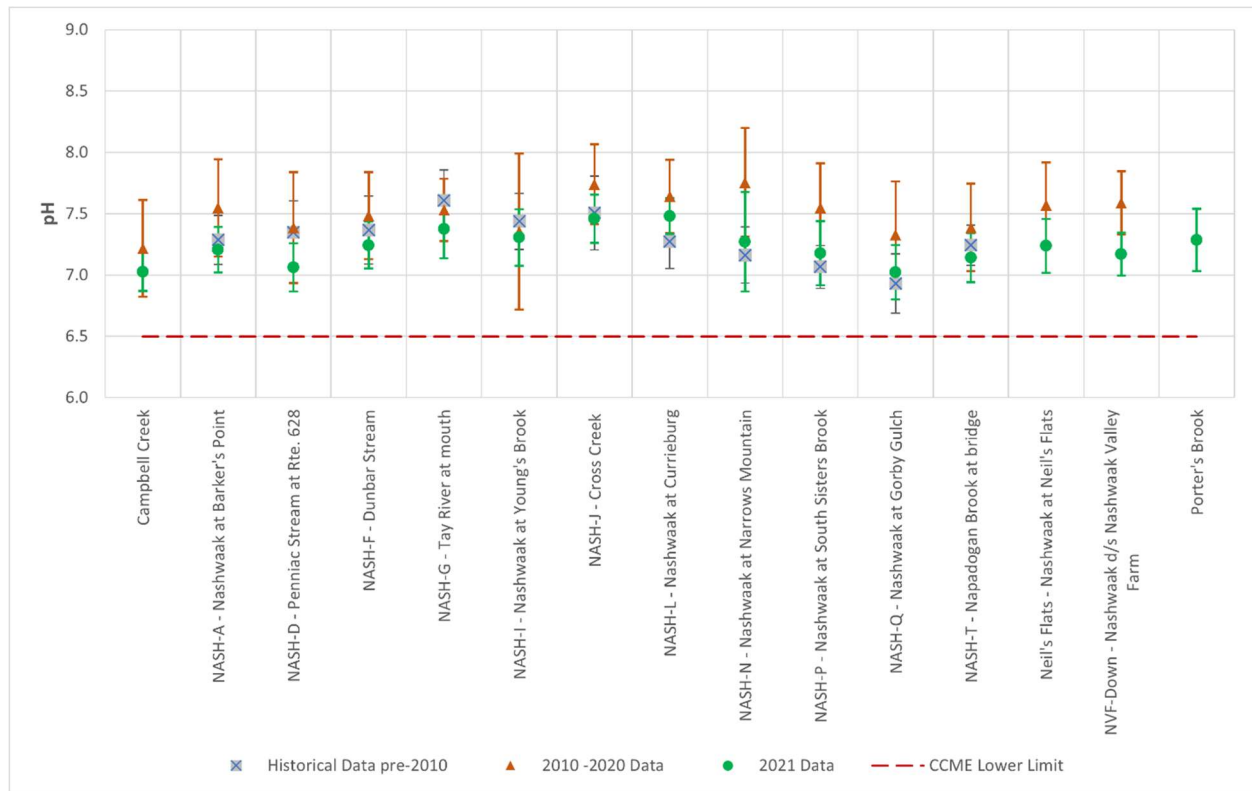
Figure 7. pH (values measured in the field) per site in the watershed (for those sites where data were available). Errors bars represent standard deviation. Historic field measurements were not available for most sites.
