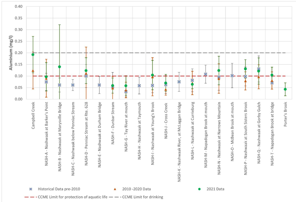
Figure 9 Aluminum content (mg/L) per site. Error bars represent standard deviation. The black dotted line represents the CCME limit of 0.2 mg/L for drinking and the red dotted line represents the CCME limit for the protection of aquatic life (0.1 mg/L).
