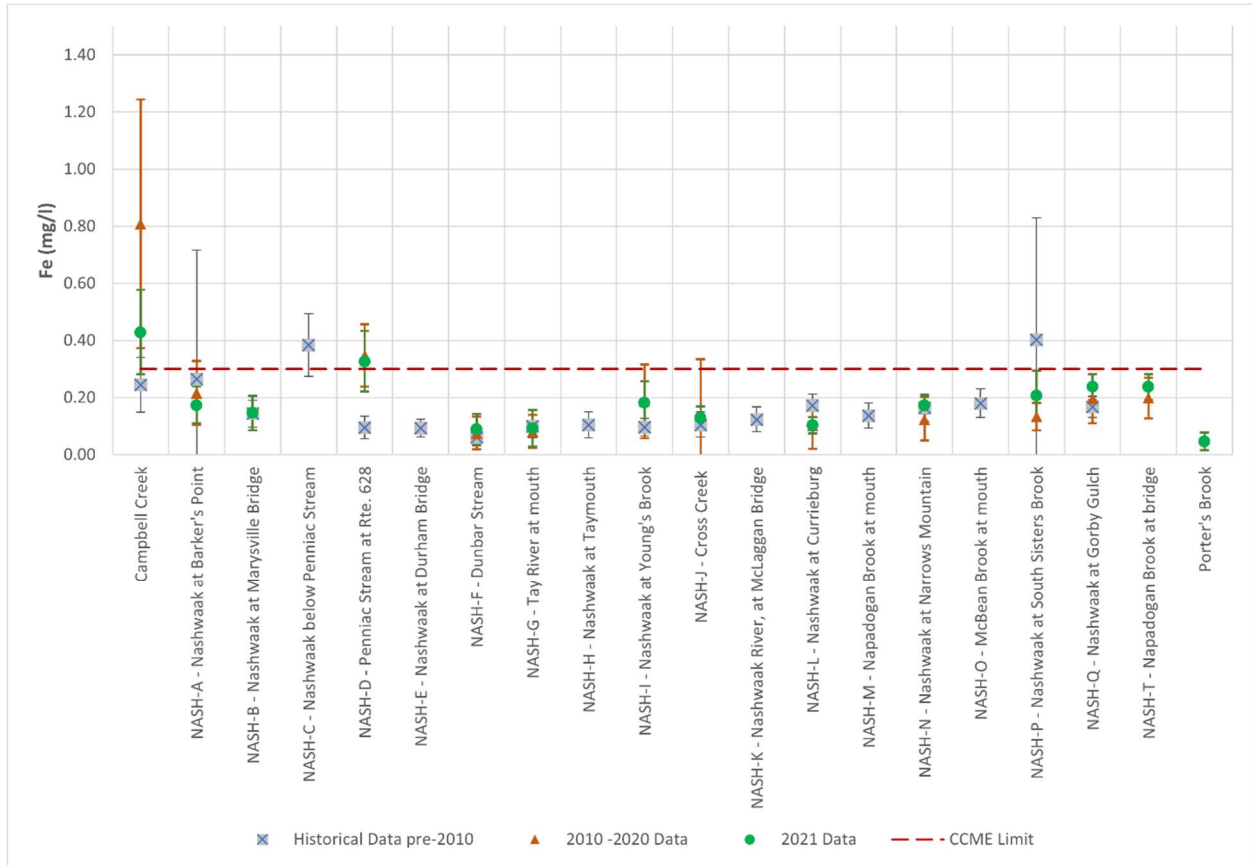
Figure 10 Mean iron content (mg/L) per site in the watershed. Error bars represent standard deviation. The dotted line represents the CCME limit of 0.3 mg/L.
