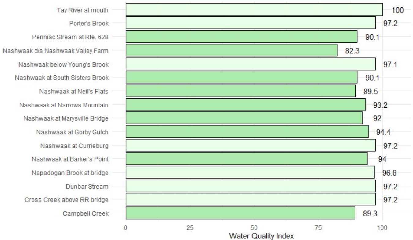
Figure 16. 2021 WQIs. Light green = Excellent, darker green = Very good
