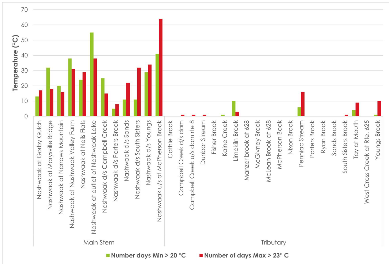
Figure 21. Number of days when minimum water temperatures exceeded 20°C and number of days when maximum daily water temperatures exceeded 23°C.
