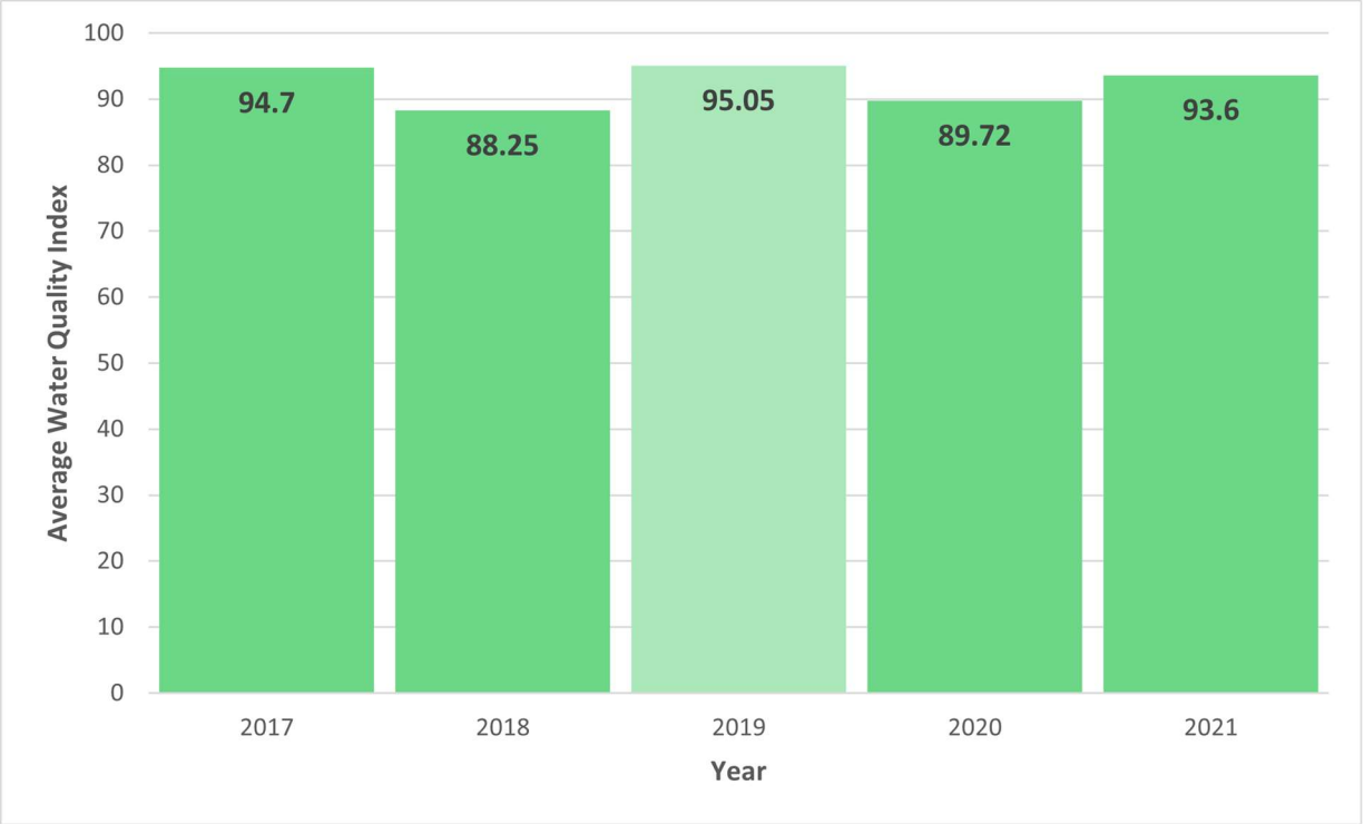
Figure 17. Comparing 2021 WQIs to previous years.
