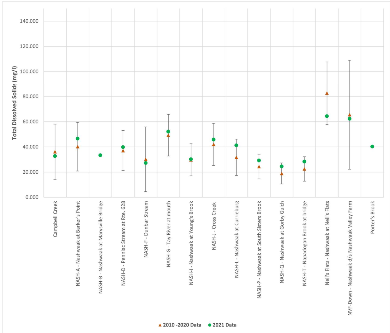
Figure 4 Mean total dissolved solid contents (mg/L) per site for the Nashwaak watershed. Error bars represent standard deviation.
