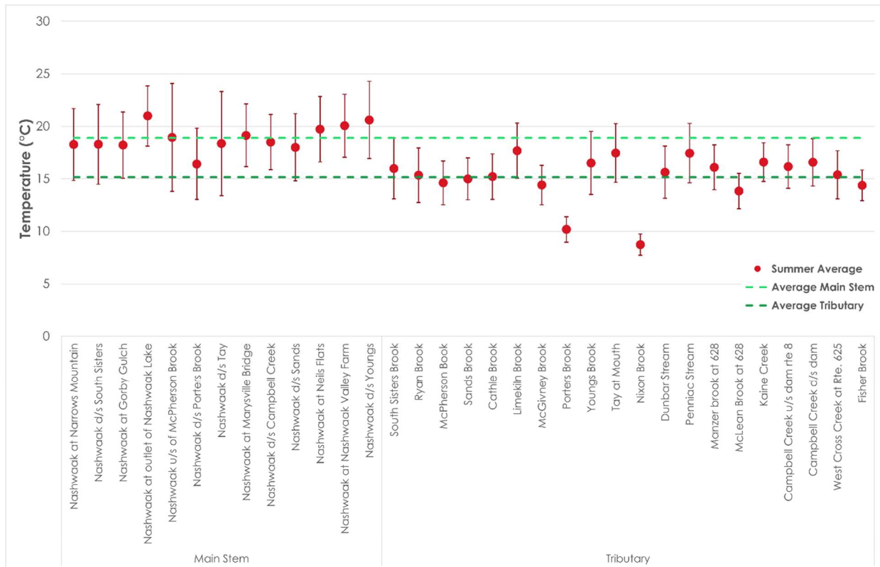
Figure 20. Average summer water temperatures (21 June to 21 September) separated by tributaries and main stem.
